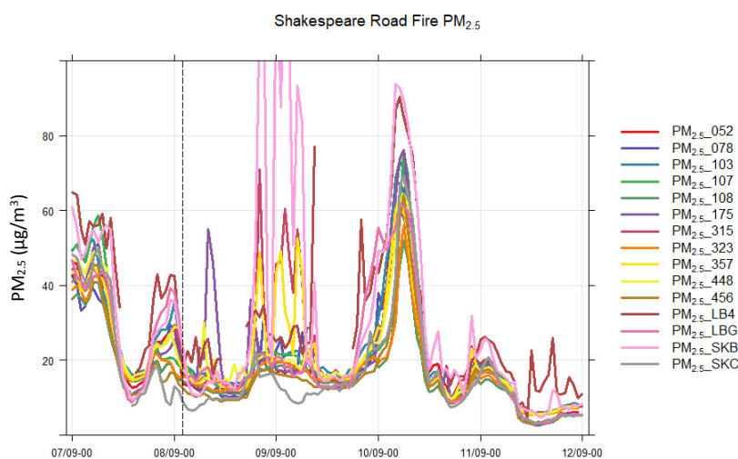
Figure 5: Figure showing data from the selected measurement sites used in this study. The dashed line shows the approximate reported start time of the fire.
